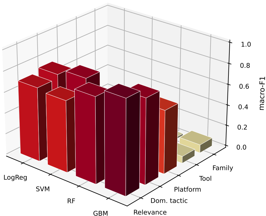
Baseline sweep in 3D: best-representation macro-F1 by task and model (stratified-random split, weak-label agreement, Section 4.3)
