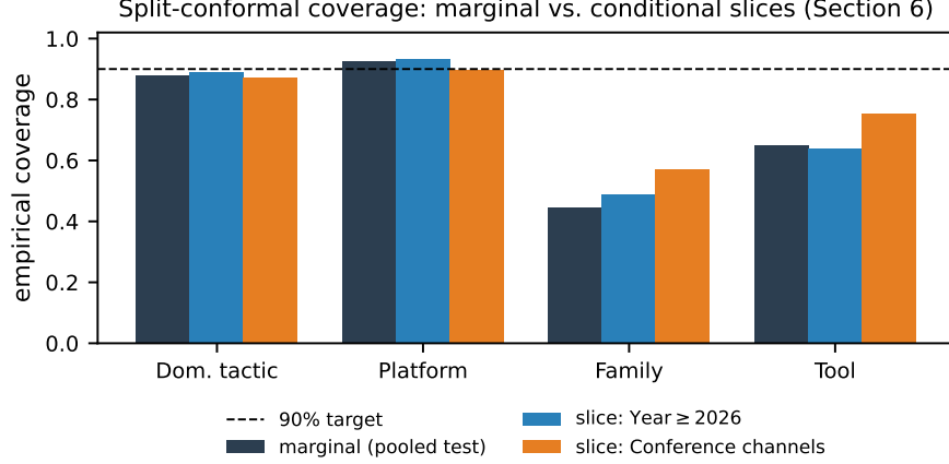
Figure 4: Empirical conformal coverage, marginal vs. the two conditional-coverage stress-test slices, against the 90% target (Table 5).
