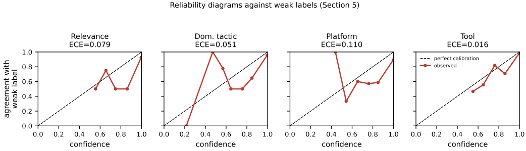
Figure 3: Reliability diagrams against weak labels, one panel per task with a usable calibration curve (Table 4). Diagonal is perfect calibration.
