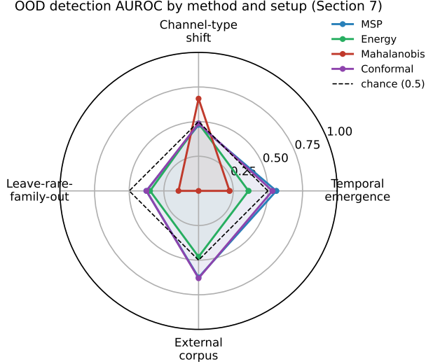
Figure 5: OOD-detection AUROC by method (color) and setup (axis), against the chance line at 0.5 (Table 6). Mahalanobis is the only method to clear chance by a wide margin, and only on one of four setups.
