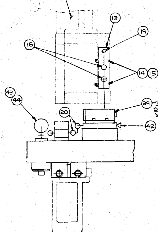
PARTIAL FRONT ELEVATION (2) GROUP 700 ONLY
