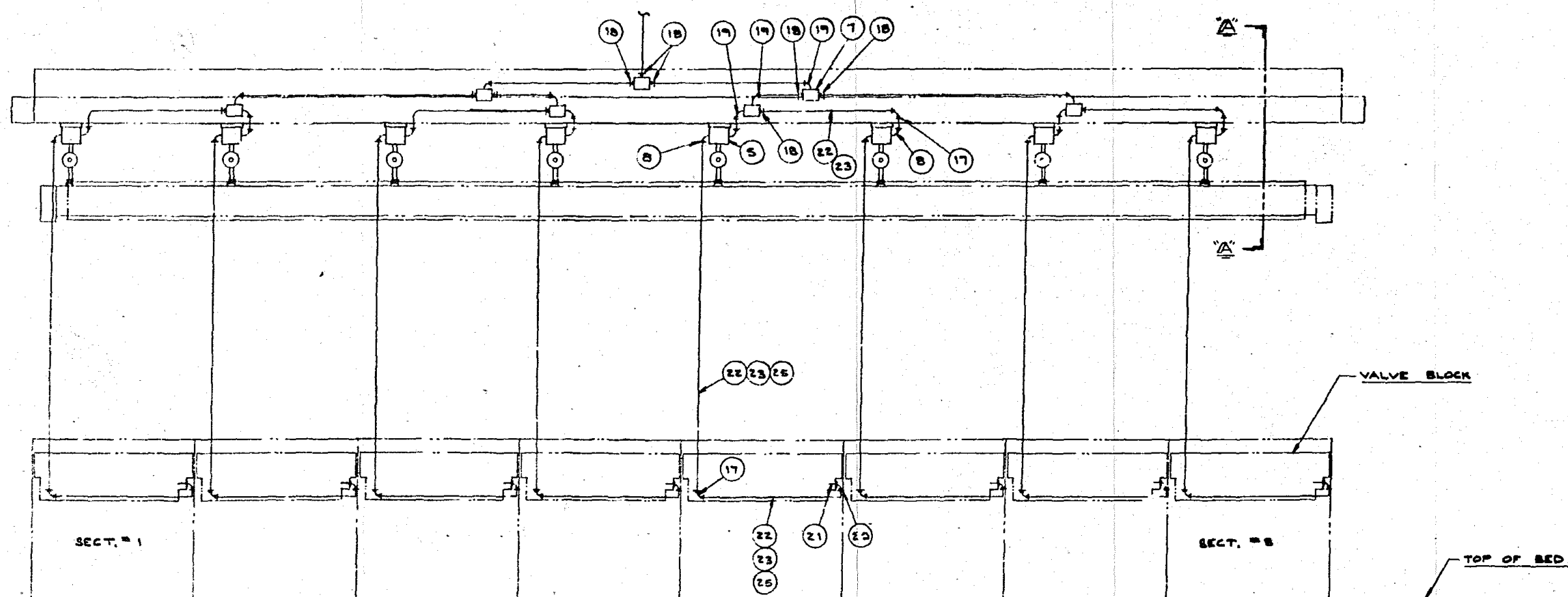
L SECT. MACH. SHOWN - GR. 701 VIEW FROM CONVEYOR SIDE
