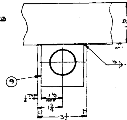
VIEW E-E TYPE B PLACES HALF SCALE
