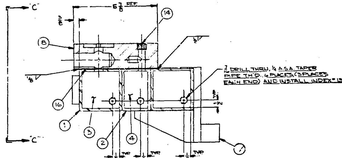
SECTION B-B TYPE 16 PLACES HALF SCALE
