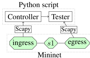
Figure 1. Experimentation setup
