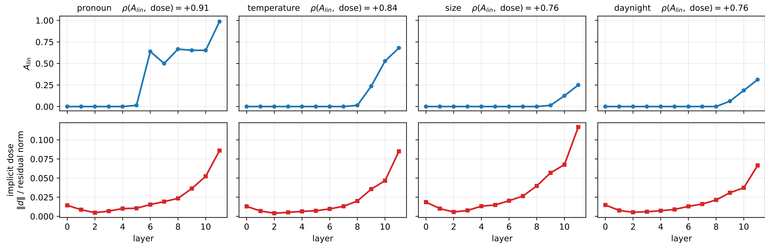
The anchor's implicit dose at coefficient 1, against its predictor, per layer
