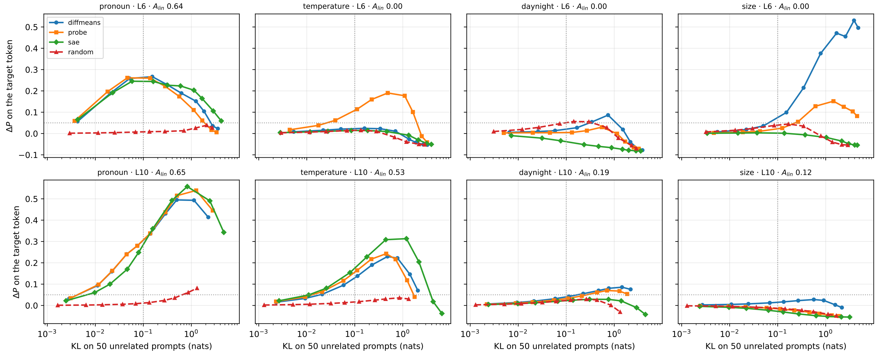
Effect against side effect: four direction sources through the dose sweep (dotted lines = the two comparison targets)
