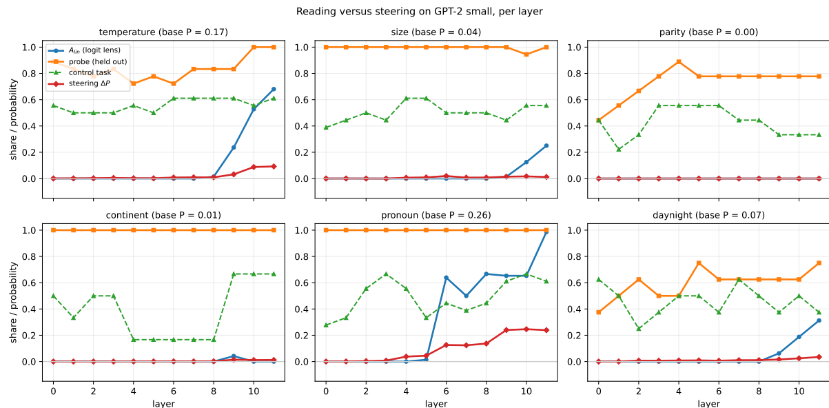
Figure 1: Reading against steering per layer, one panel per family. A_{lin} (circles) rises late; the probe (squares) is flat and high wherever the family has one template; the control task (triangles) shows the probe is not merely memorising; steering \Delta P (diamonds) follows A_{lin} , not the probe. Source: notebooks/07_reading_vs_steering.ipynb .
