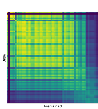
(a) RSA of the pretrained and non-pretrained models.
