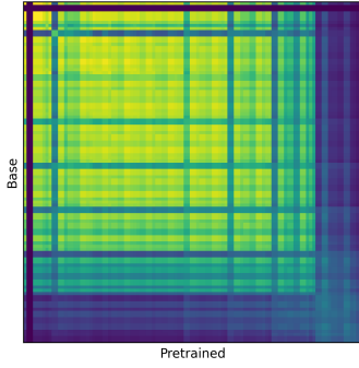
(a) RSA of pre-trained and non-pre-trained models.
