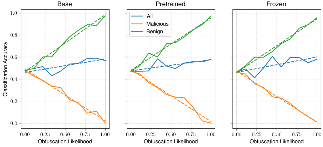
(a) File-level performance
