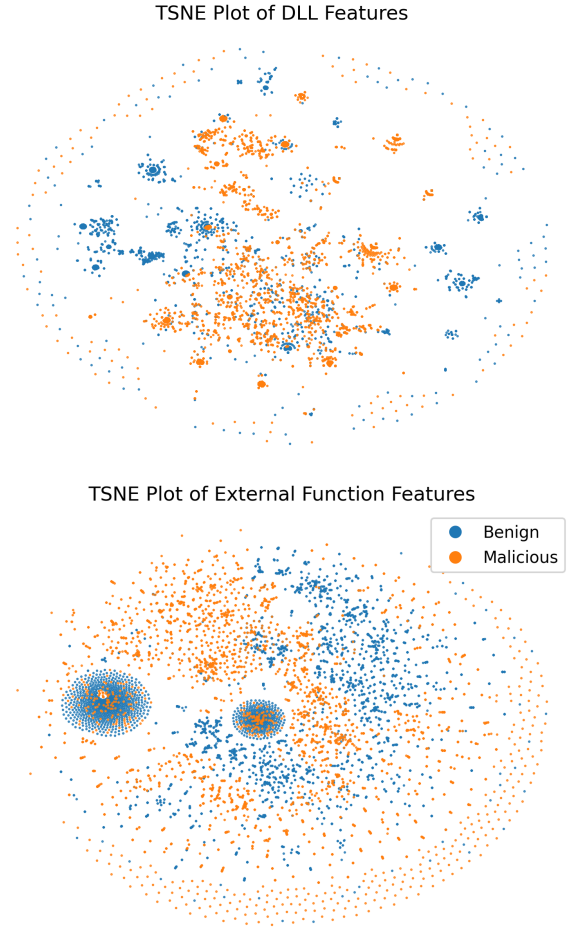
Figure 14: Comparison between the functions and DLLs used by malicious and benign programs.
