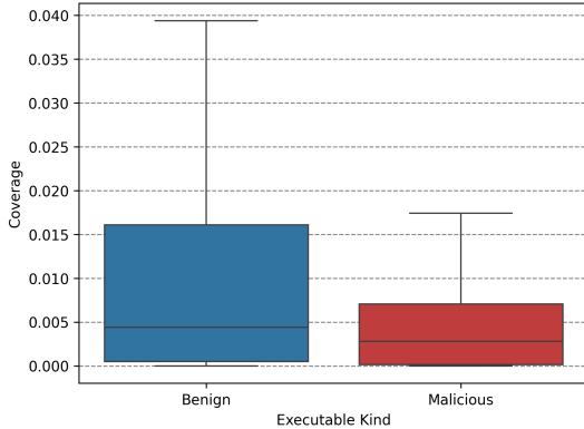
(b) Distribution of code analysis coverage across classes.
