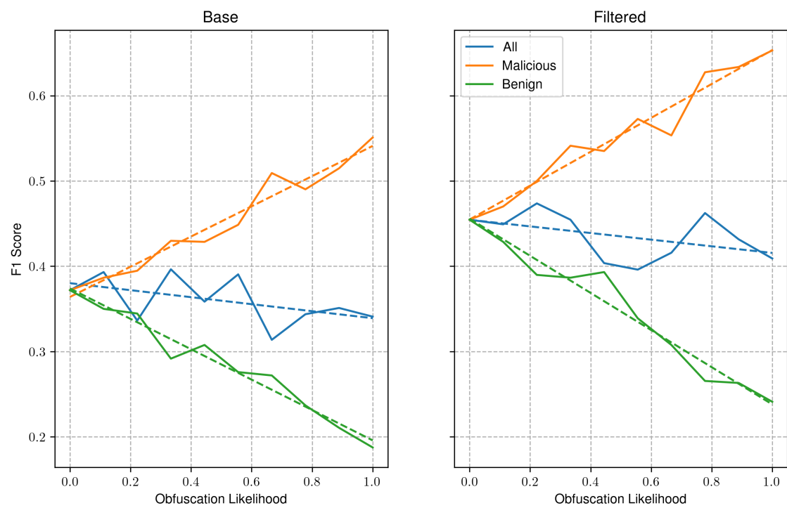
Figure 22: Impact of obfuscation on the F1 score of our image classification malware detection model.
