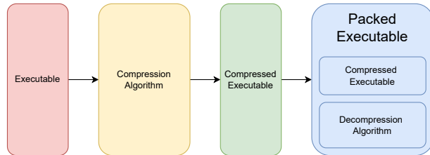
Figure 3: Binary packing for compression and obfuscation of executables
