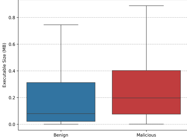
Figure 8: Distribution of executable size in the filtered dataset
