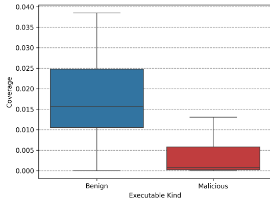
Figure 16: Extent of obfuscation between classes in the secondary dataset.
