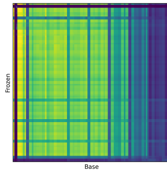
(c) RSA of the frozen and non-pretrained models.
