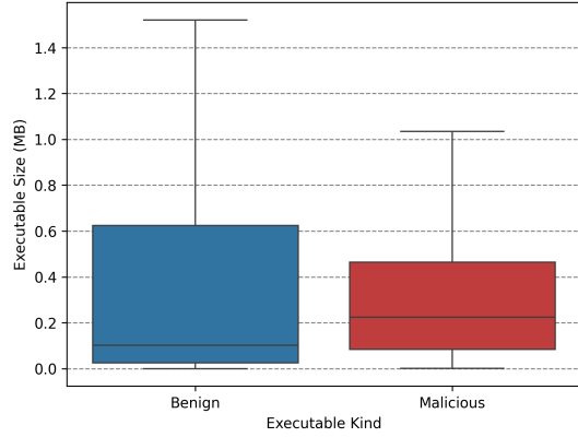
(a) Distribution of executable size across classes.
