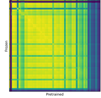
(b) RSA of the pretrained model and our pretrained model with frozen attention layer weights.
