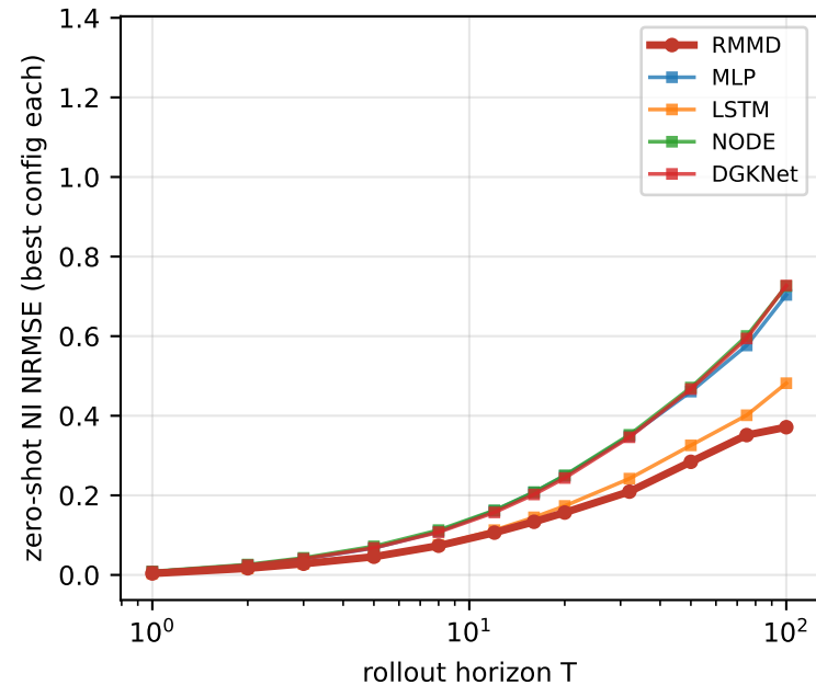
EAST
