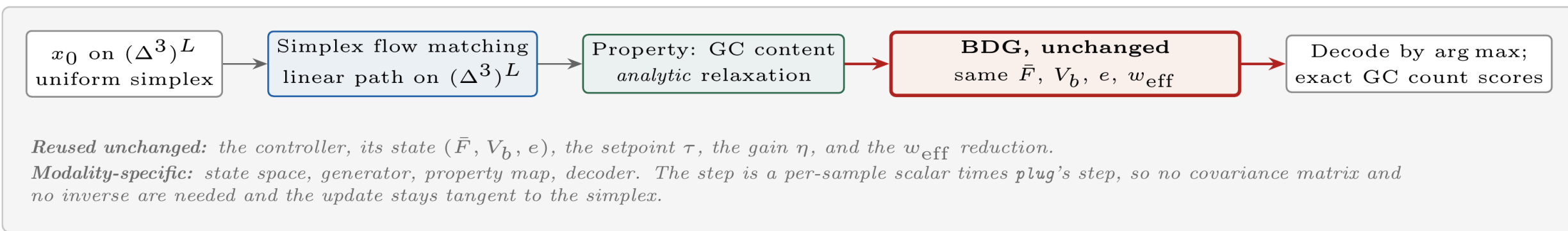
(b) Modality 2: DNA enhancers on the probability simplex (\Delta^3)^L
