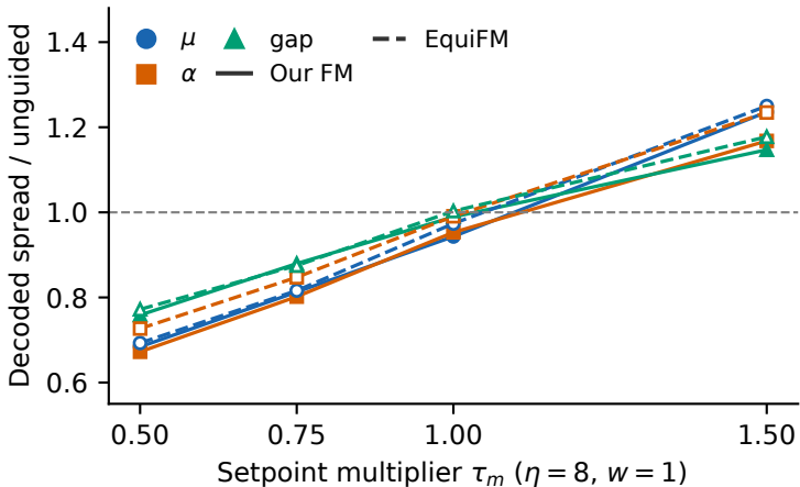
(a) QM9: setpoint changes spread
