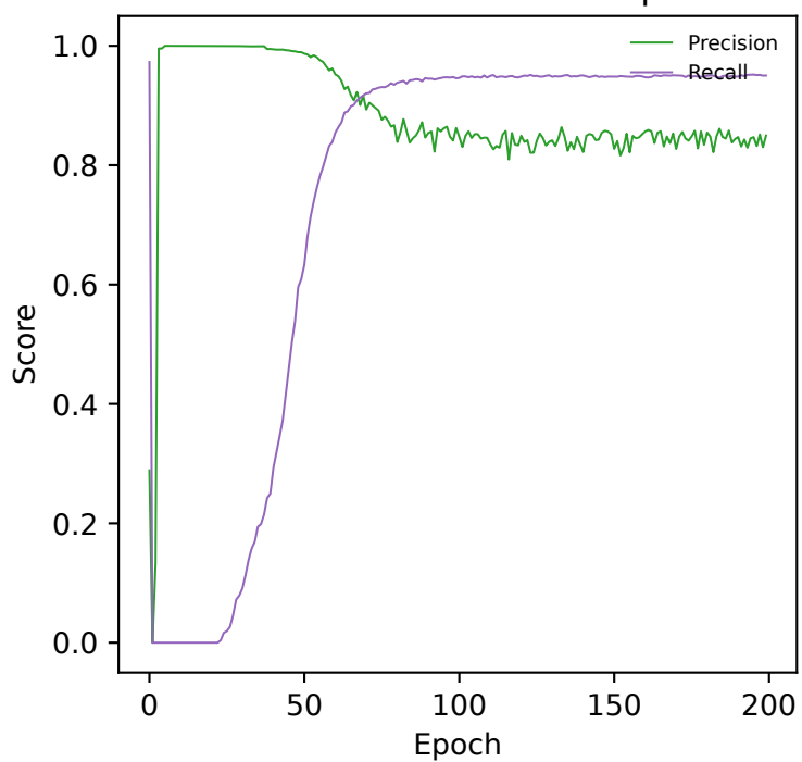
Precision and Recall over Epochs
