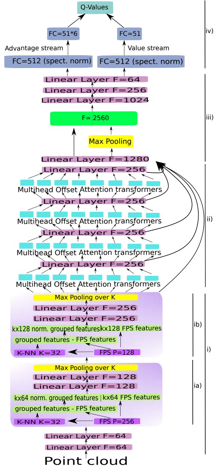
Fig. 2. The network architecture utilized for the experiment, where F denotes the feature vector's length and FC denotes a fully connected layer. Dashed lines represent concatenated layers. i) Two embedding blocks are used: ia) and ib). ii) The offset multihead attention block. iii) From PointNet, a component of the segmentation network was incorporated to preserve spatial information by performing max pooling on the points, copying them N times, and concatenating them with the original tensor. iv) A distributional and dueling network structure with spectral normalization.
