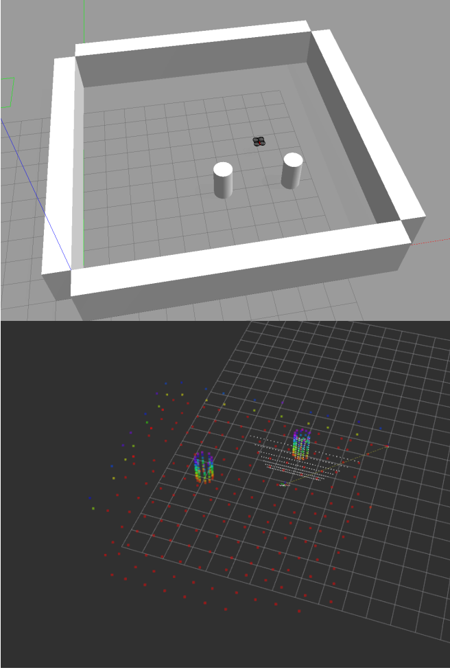
Fig. 1. Top: The environment with 2 cylinders, where our sensor is represented by the drone icon. Bottom: A point cloud of the environment with two cylinders placed in different locations than in the top figure. The white points represent the new incoming observation at time step t of the agent, prior to its concatenation with the previous point cloud S_t .
