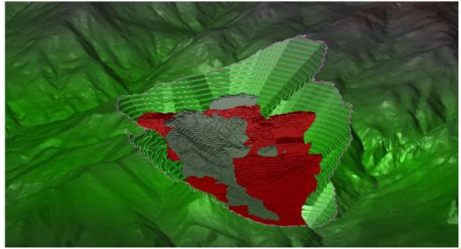
Mine Design - Open Pit (Sungai Mak)
