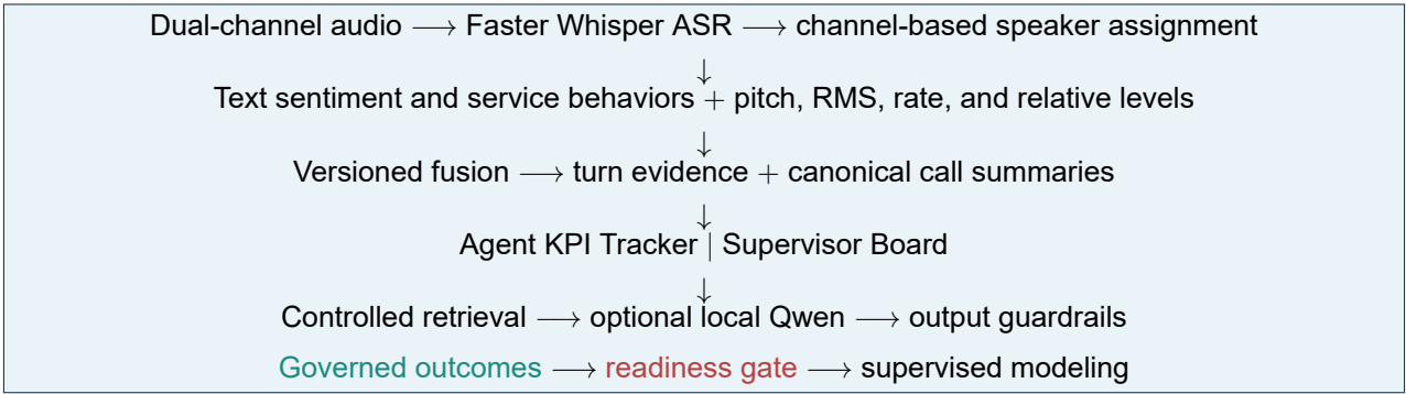
Figure 1: Models produce bounded signals; contracts and guardrails control business-facing output.
