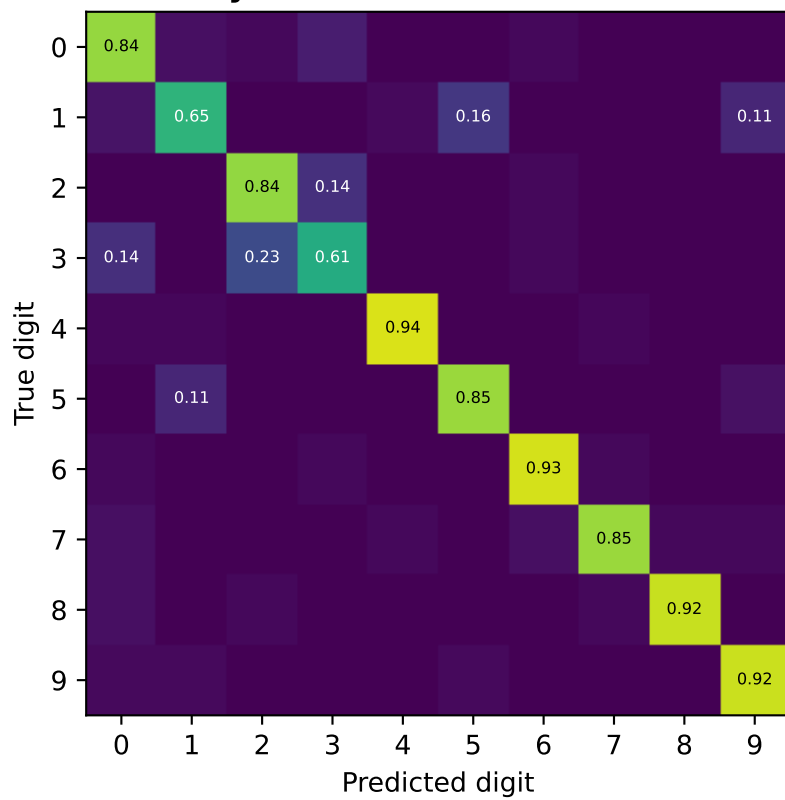
(c) Test confusion Accuracy = 0.840
