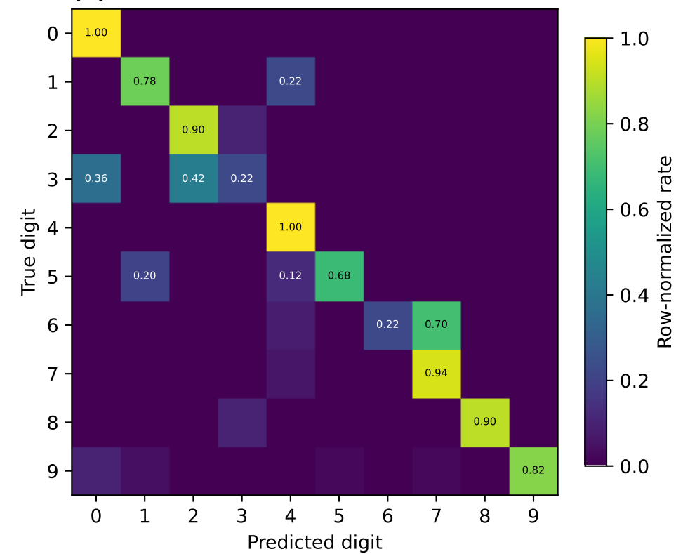
(e) Conv1D test confusion
