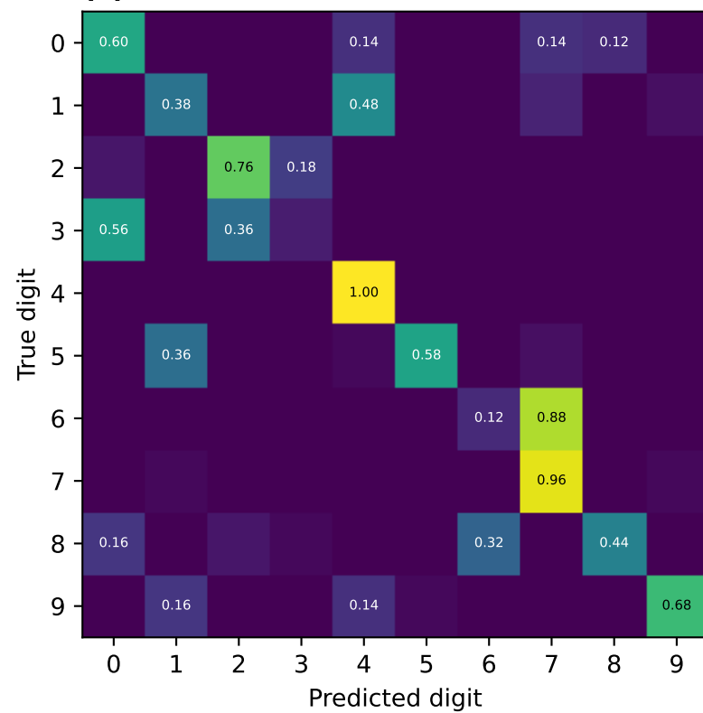
(c) Pooled EGFN test confusion
