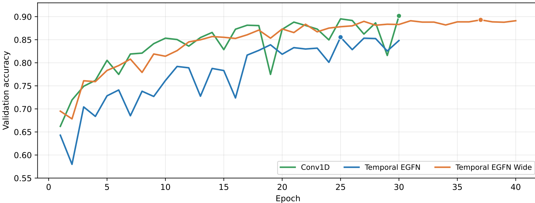
(a) Official validation split
