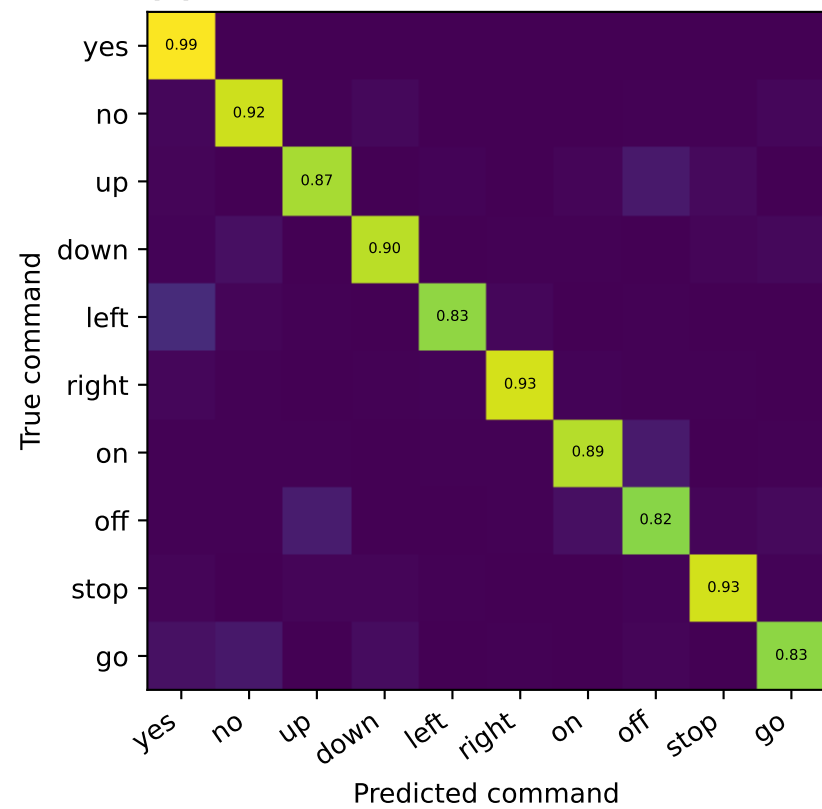
(c) Conv1D test confusion
