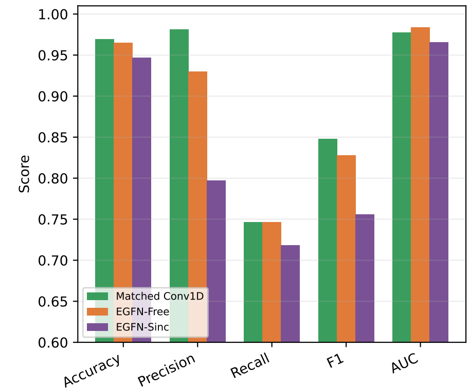
(c) Calibrated test metrics
