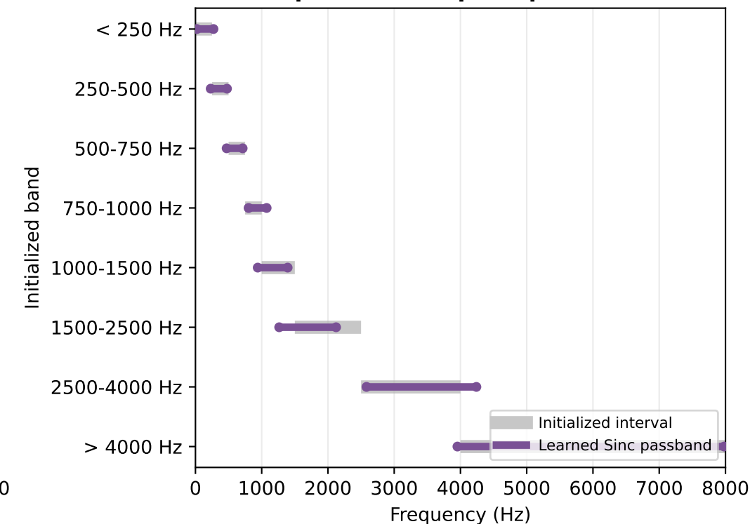
(f) Sinc preserves explicit passbands
