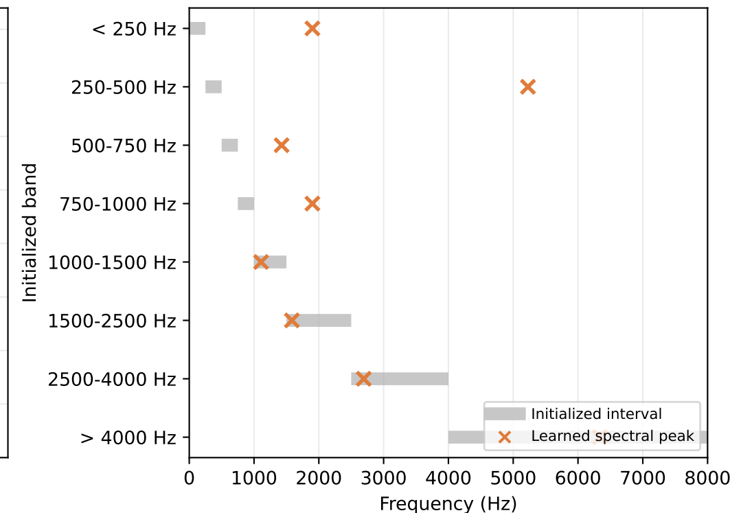
(e) Free FIR kernels lose band constraint
