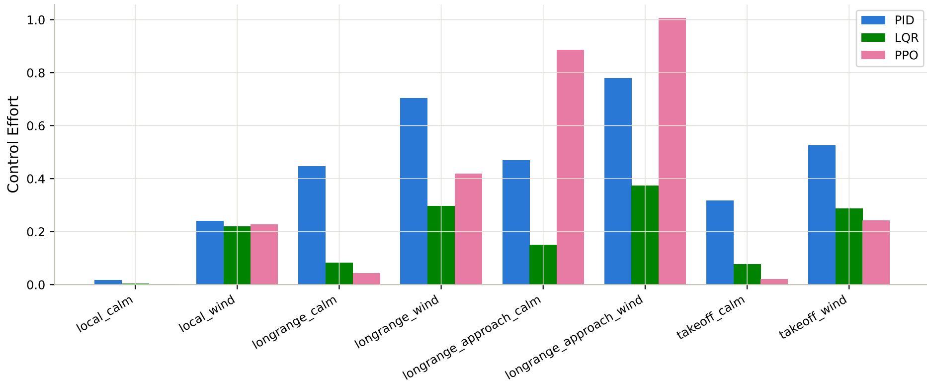
Control Effort by Scenario
