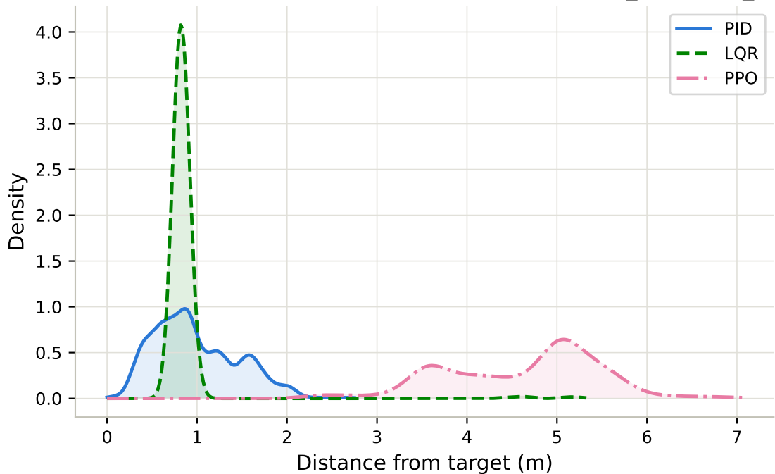
Steady-State Tracking Error Distribution - longrange_approach_wins
