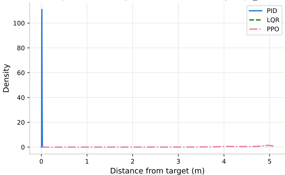
Steady-State Tracking Error Distribution - longrange_calm
