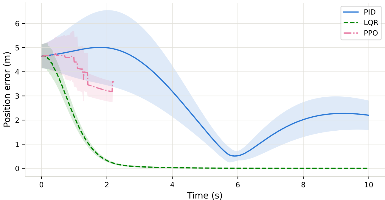
Tracking Error Over Time (mean \pm std, n=20) - longrange_approach_calm
