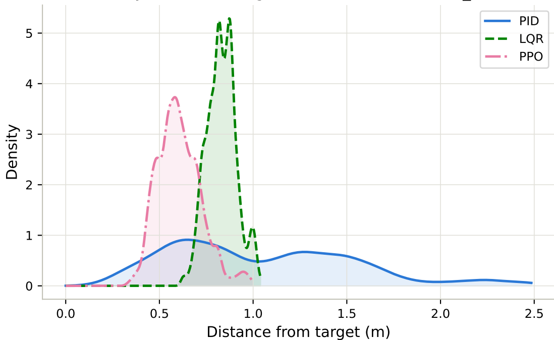
Steady-State Tracking Error Distribution - local_wind
