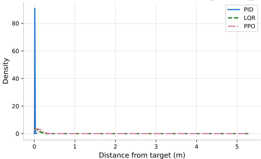
Steady-State Tracking Error Distribution - longrange_approach_calm
