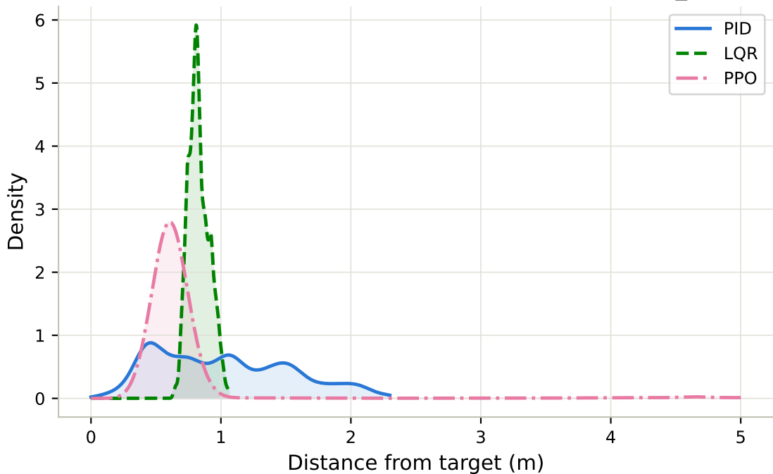
Steady-State Tracking Error Distribution - longrange_wind
