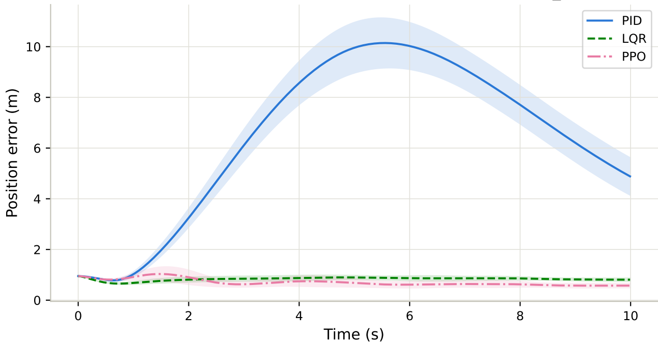
Tracking Error Over Time (mean \pm std, n=20) - takeoff_wind
