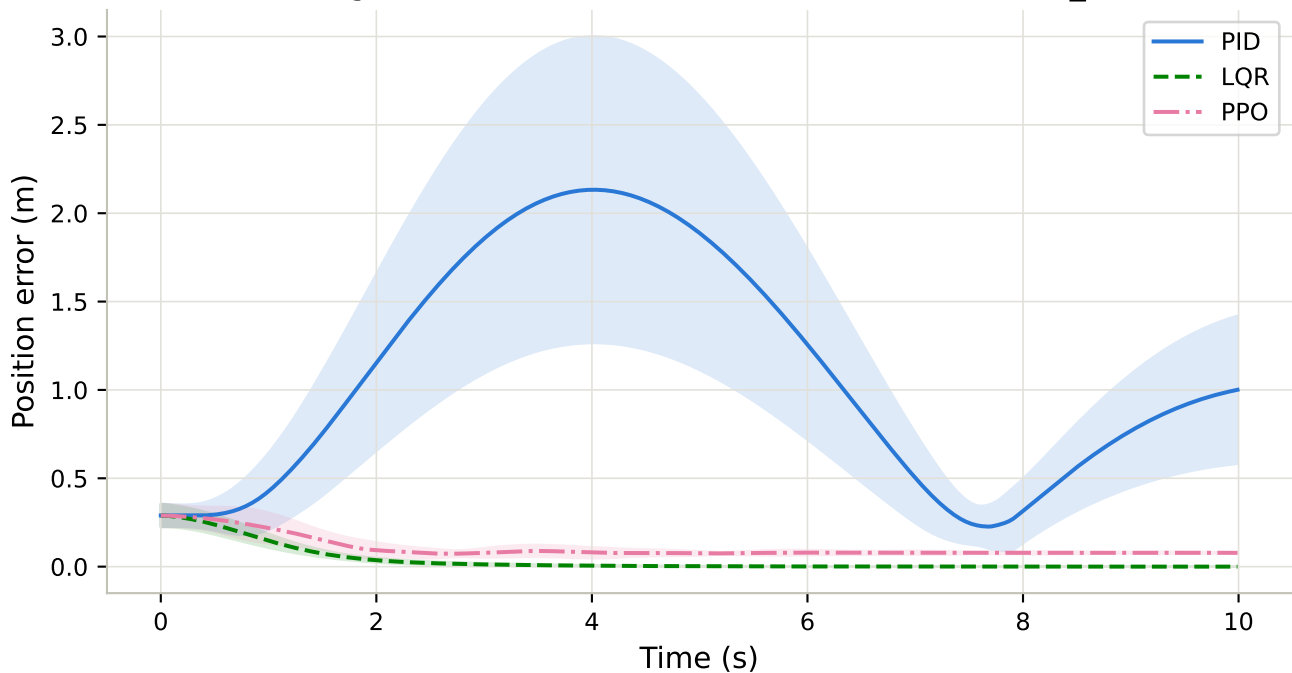
Tracking Error Over Time (mean \pm std, n=20) - local_calm
