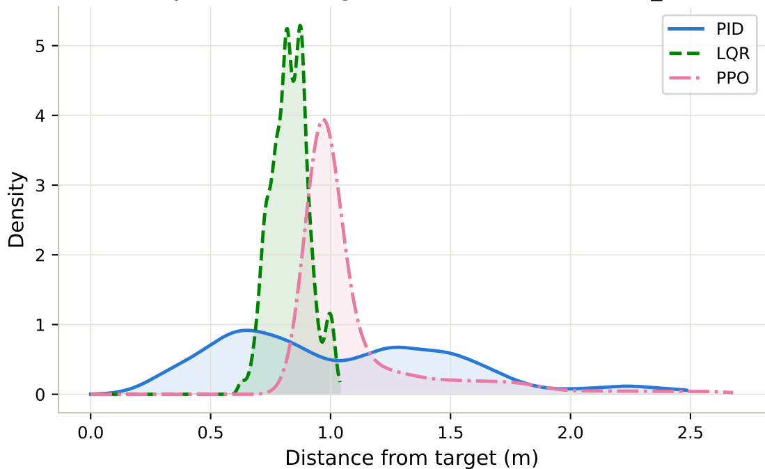
Steady-State Tracking Error Distribution - takeoff_wind
