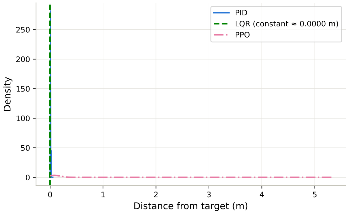
Steady-State Tracking Error Distribution - longrange_approach_calr
