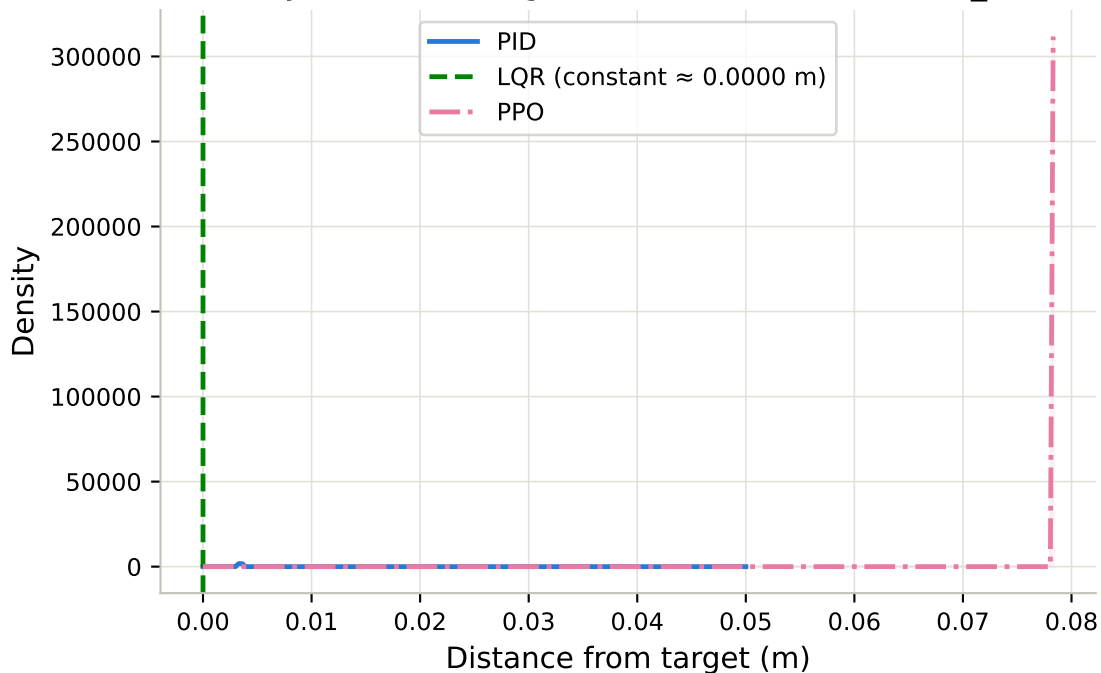
Steady-State Tracking Error Distribution - takeoff_calm
