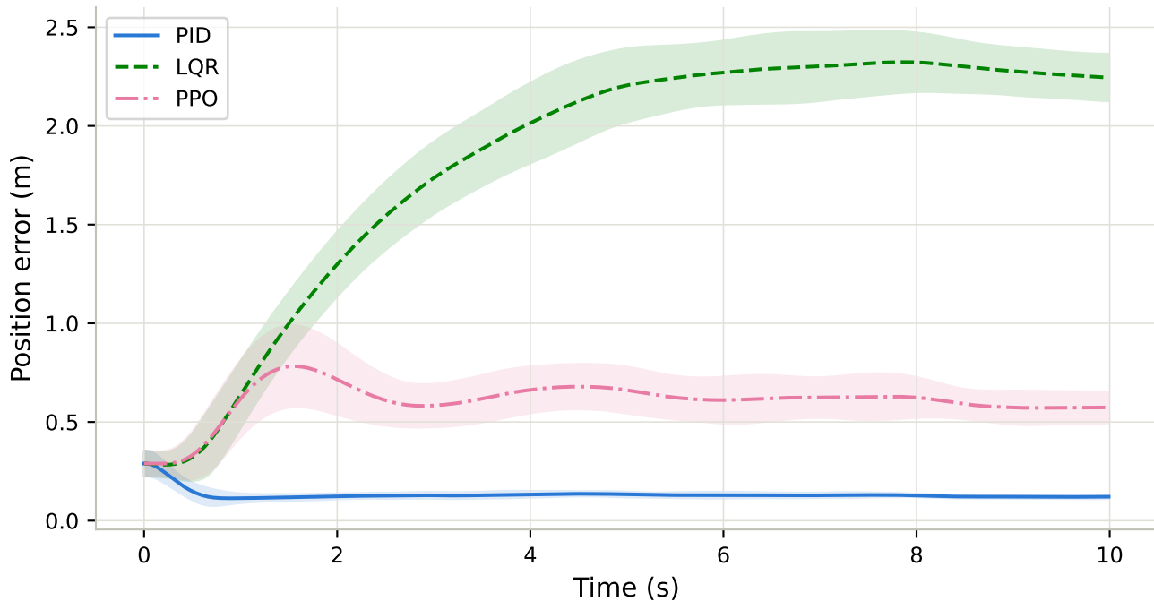
Tracking Error Over Time (mean \pm std, n=20) - local_wind
