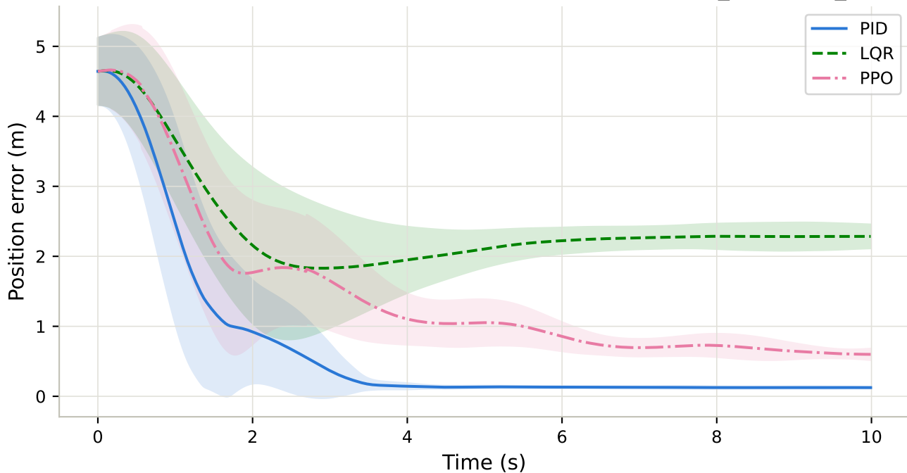
Tracking Error Over Time (mean \pm std, n=20) - longrange_approach_wind
