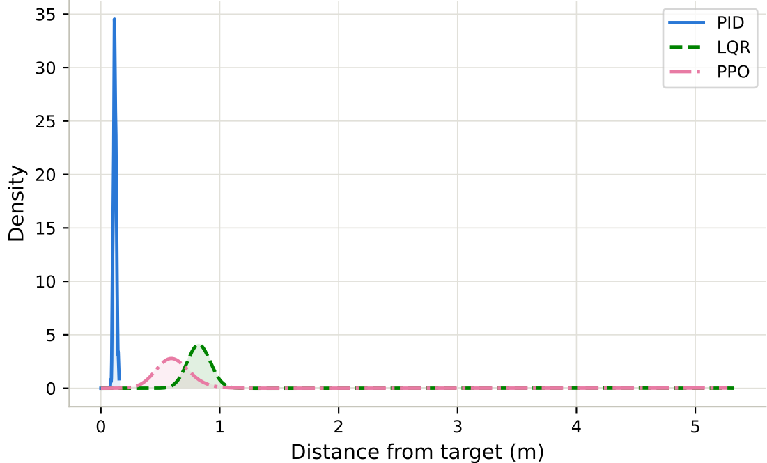
Steady-State Tracking Error Distribution - longrange_approach_winc
