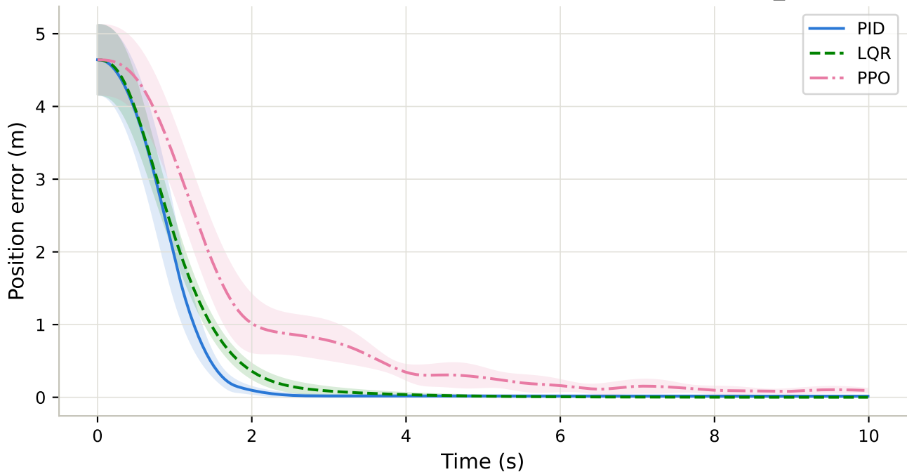
Tracking Error Over Time (mean \pm std, n=20) - longrange_calm
