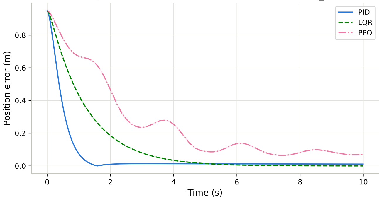
Tracking Error Over Time (mean \pm std, n=20) - takeoff_calm
