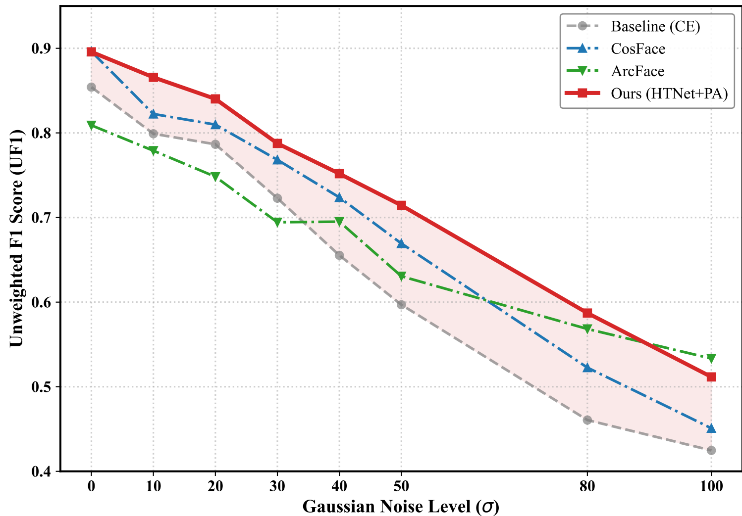
Noise Robustness Comparison
