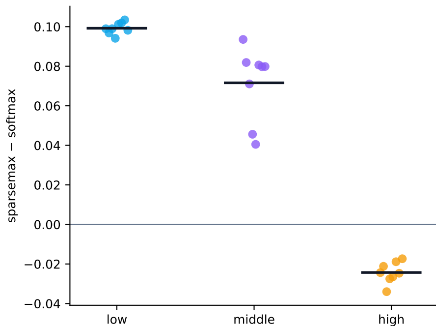
D Paired dimension-AUC difference
