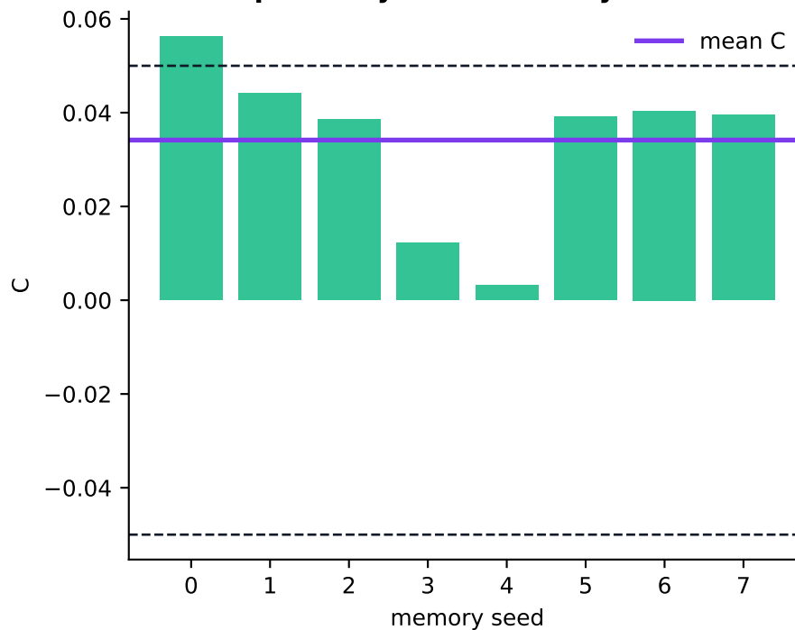
E Exploratory interaction by old seed
