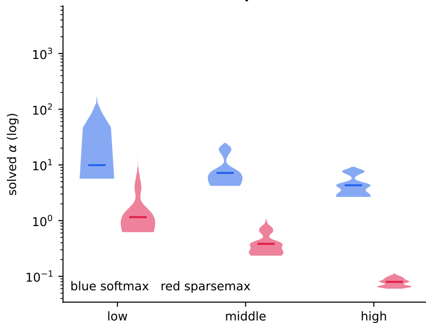
A Per-cue sharpness solutions
