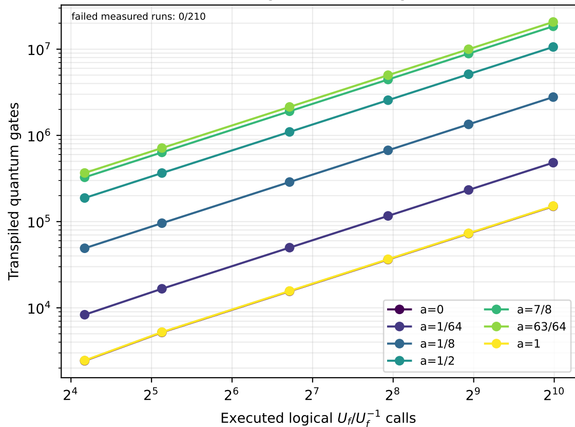
Shot-weighted schedule gates
