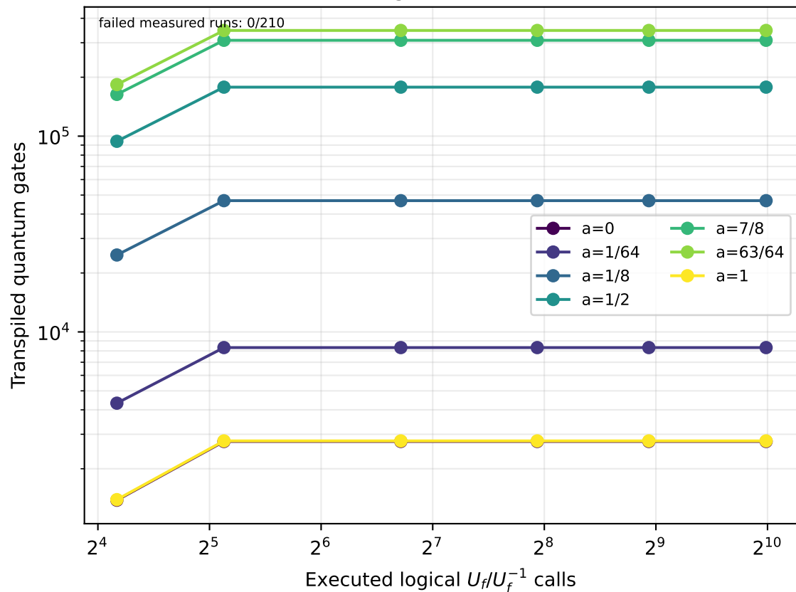
Maximum gates in one circuit
