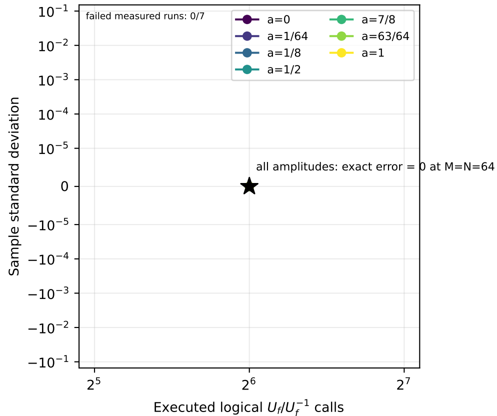
Exact finite-table control
