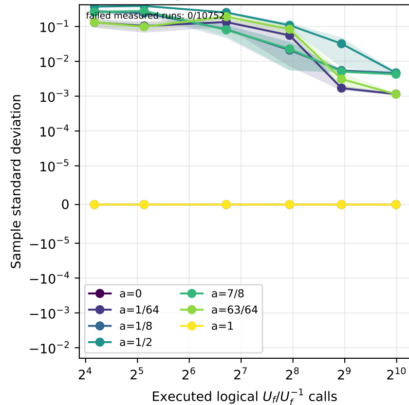
Analytical finite-shot MLAE
