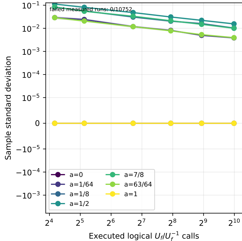
Classical Monte Carlo
