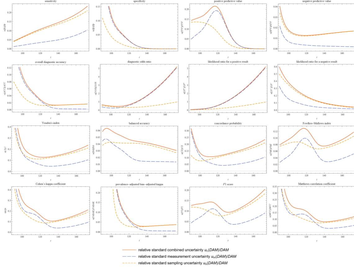
Figure 7. Relative standard sampling, measurement, and combined uncertainty of the sixteen DAMs versus threshold t , with the settings of the program in Table 7.
