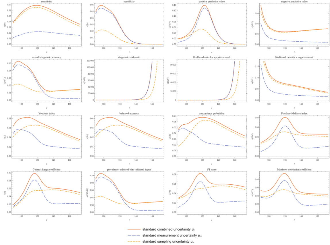
Figure 6. Standard sampling, measurement, and combined uncertainty of the sixteen DAMs versus threshold t , with the settings of the program in Table 7.
