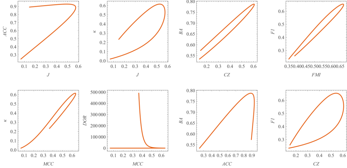
Figure 5. Plots of overall diagnostic accuracy ( ACC ) and Cohen's kappa coefficient ( \kappa ) versus Youden's index ( J ), balanced accuracy ( BA ) versus concordance probability ( CZ ), F1 score ( F1 ) versus Fowlkes–Mallows index ( FMI ), Cohen's kappa coefficient ( \kappa ) and diagnostic odds ratio ( DOR ) versus Matthews correlation coefficient ( MCC ), balanced accuracy ( BA ) versus overall diagnostic accuracy ( ACC ), and F1 score ( F1 ) versus concordance probability ( CZ ), with the settings of the program in Table 7.
