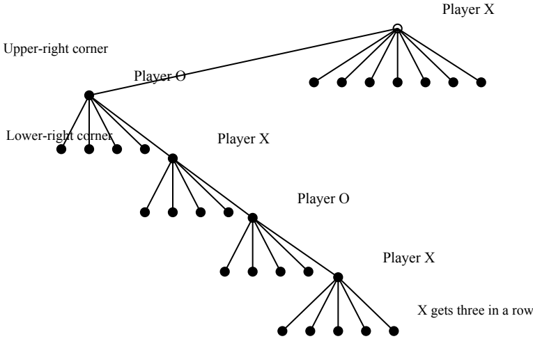
Figure 7.C.2. Part of the extensive form for Tick-Tack-Toe.
