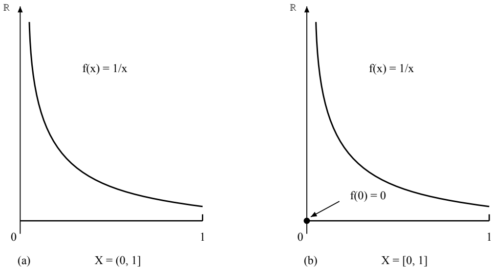
Figure M.F.3. Indispensability of the continuity and compactness assumptions for the existence of a maximizer. (a) A continuous function with no maximizer on a noncompact domain. (b) A discontinuous function with no maximizer on a compact domain.
