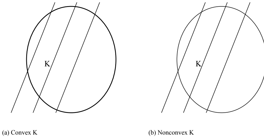
Figure 3.F.2. A closed set is convex if and only if it equals the intersection of the half-spaces that contain it: (a) convex K ; (b) nonconvex K .
