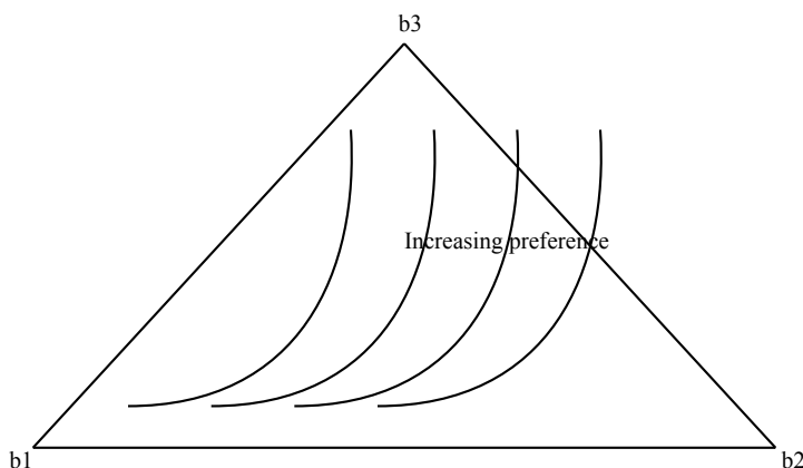
Figure 6.B.8 An indifference map for induced preferences over lotteries on B = \{b_1, b_2, b_3\} .
