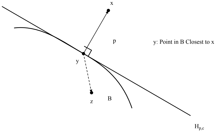
Figure M.G.5. The separating hyperplane theorem.
