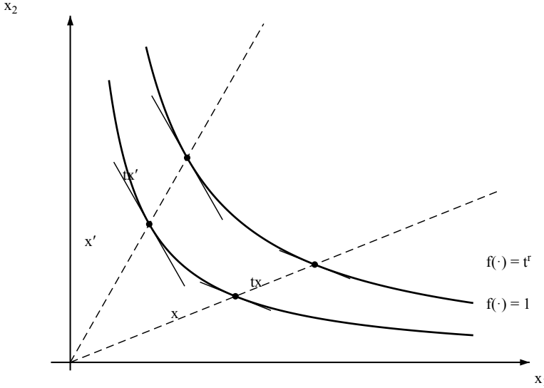
Figure M.B.1 The level sets of a homogeneous function.
