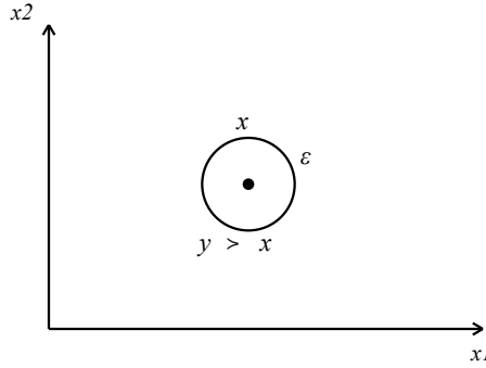
Figure 3.B.1. The test for local nonsatiation.
