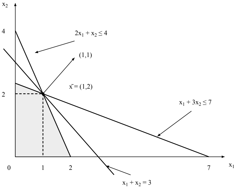
Figure M.M.1 A linear programming problem (the primal).
