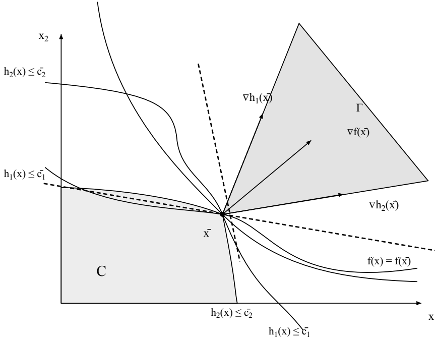
Figure M.K.2 Necessity of the Kuhn–Tucker conditions.
