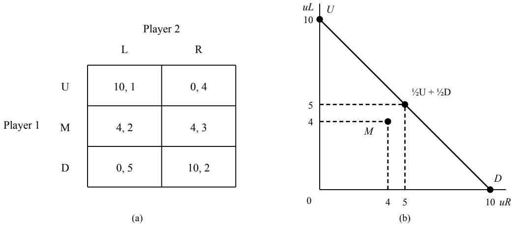
Figure 8.B.5. Domination of a pure strategy by a randomized strategy.
