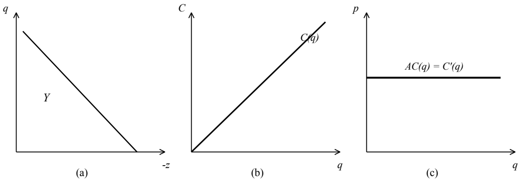
Figure 5.D.2. A constant returns to scale technology. (a) Production set. (b) Cost function. (c) Average cost, marginal cost, and supply.
