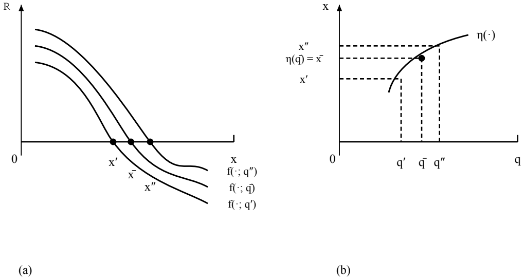
Figure M.E.1. A locally solvable equation. (a) Solutions of f(x; q) = 0 near (\bar{x}, \bar{q}) . (b) The graph of \eta(\cdot) .
