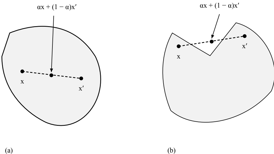
Figure M.G.1. Convex and nonconvex sets. (a) A convex set. (b) A nonconvex set.
