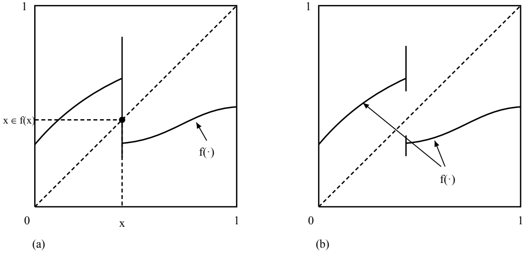
Figure M.I.2. Kakutani's fixed point theorem. (a) A fixed point exists. (b) The convex-valuedness assumption is indispensable.
