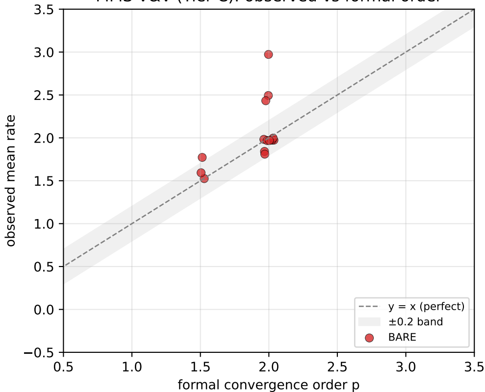
MMS V&V (Tier C): observed vs formal order
