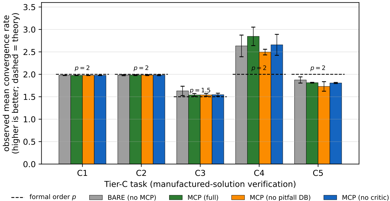
Tier C: observed convergence rates per task and condition bars are means over 3 seeds; error bars are seed standard deviation
