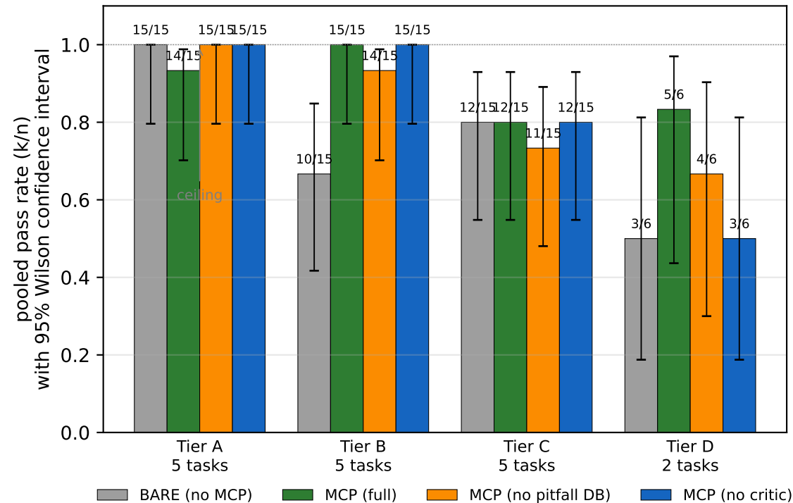
Pass rate by difficulty tier n=15 cells per tier per condition (5 tasks × 3 seeds), except Tier D where n=6
